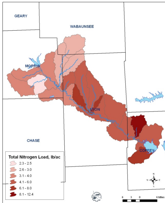
Figure 16. Total Nitrogen Load, pounds/acre as Indicated by SWAT.
