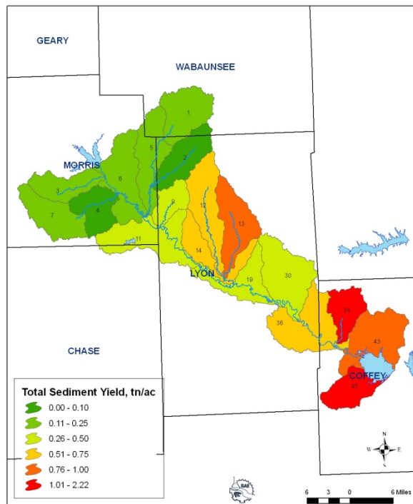
Figure 17. Total Sediment Yield, tons/acre as Indicated by SWAT.
