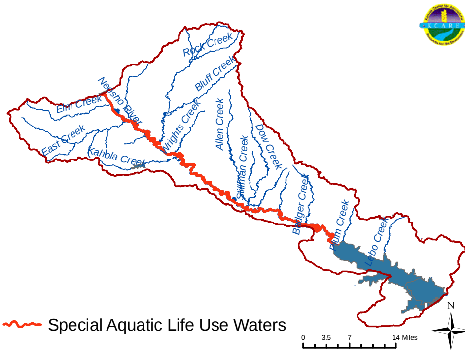
Figure 6. Special Aquatic Life Use Waters in the Watershed. 6 Kansas Department of Health and Environment.
