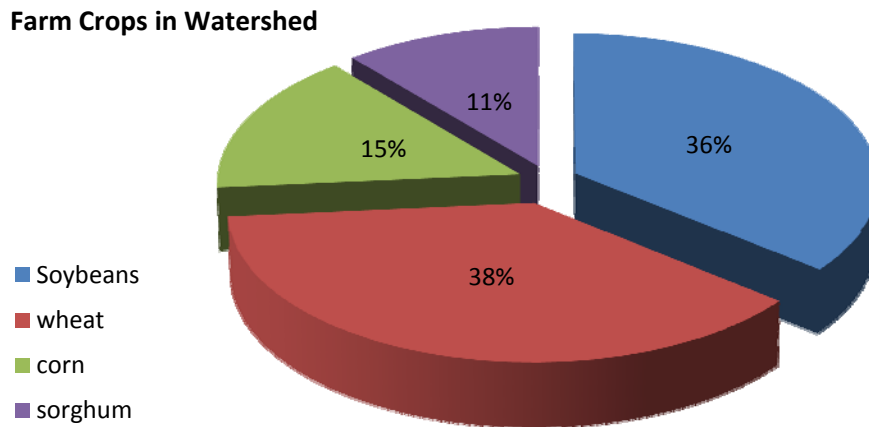
Figure 38. Farm Crops. Total farm crops in the counties of the watershed by percentage. 2007 Census of Agriculture, USDA NASS. 40
