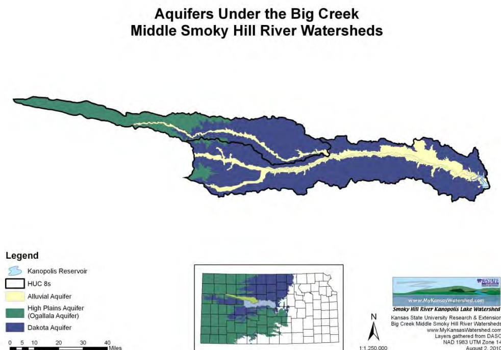
Figure 9. Aquifers under the BCMSHRW.
